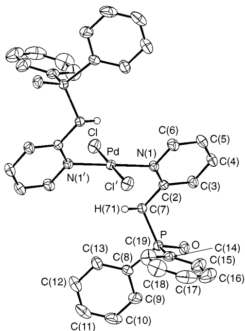
Fig. 3 An ORTEP view of compound 6 . Primed atoms are related to unprimed ones by the symmetry operation 1 - x, -y, 1 - z . Ellipsoids are as in Fig. 1.
